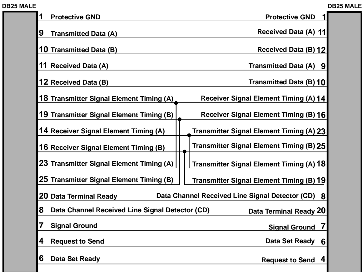
Figure 3 - 12 V.35 Null-Modem Cable
