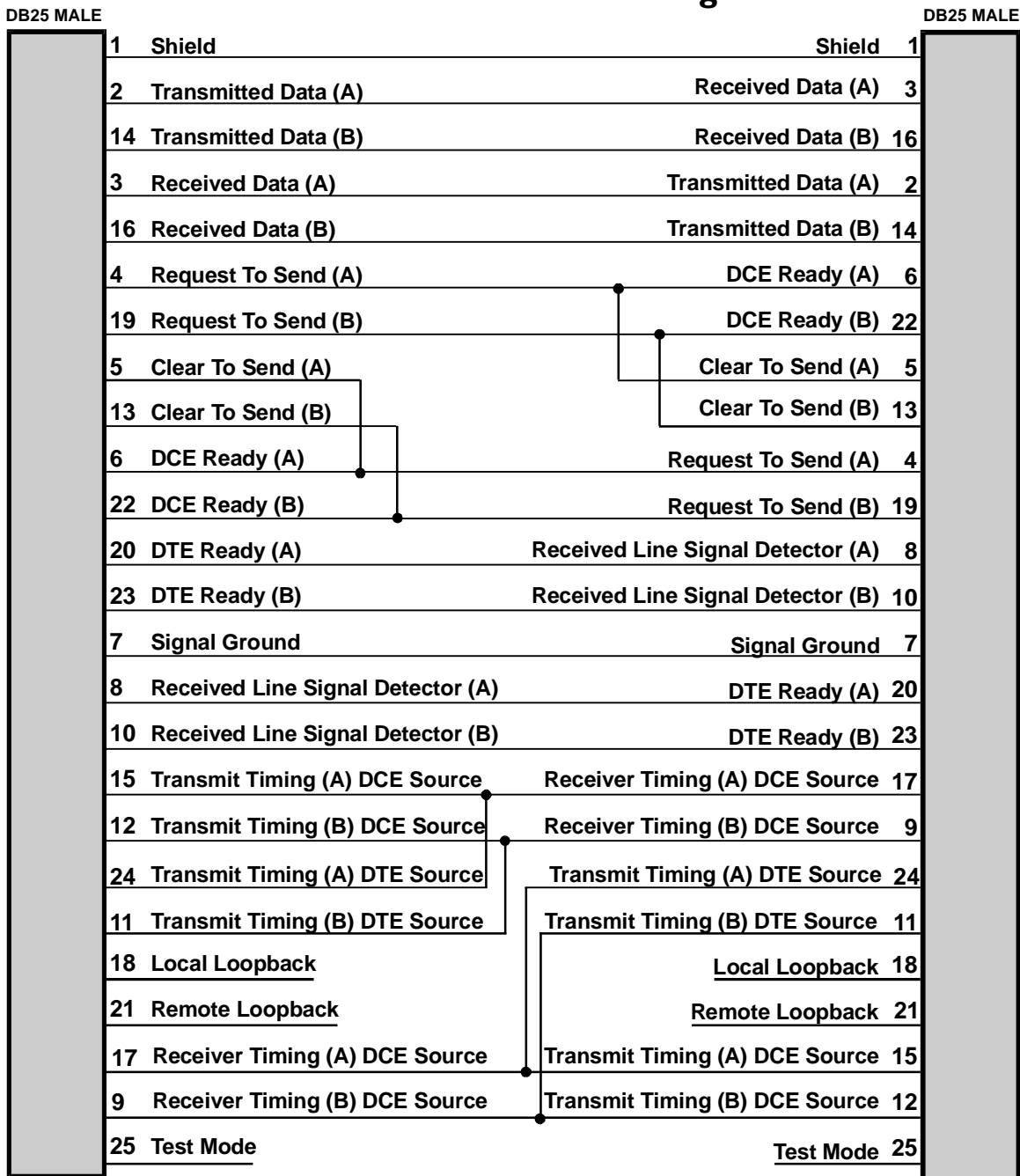
Figure 3 – 13 RS530 Null-Modem Cable
