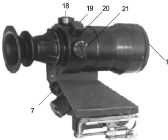
Figure 2. Sight (right side view)
