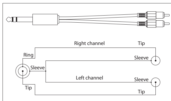
1/4" TRS to stereo RCA
