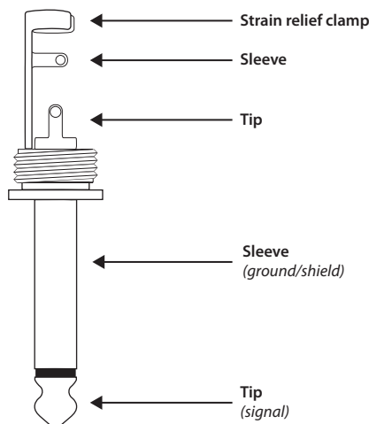
Unbalanced 1/4" TS connector
