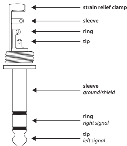
1/4" TRS headphones connector
