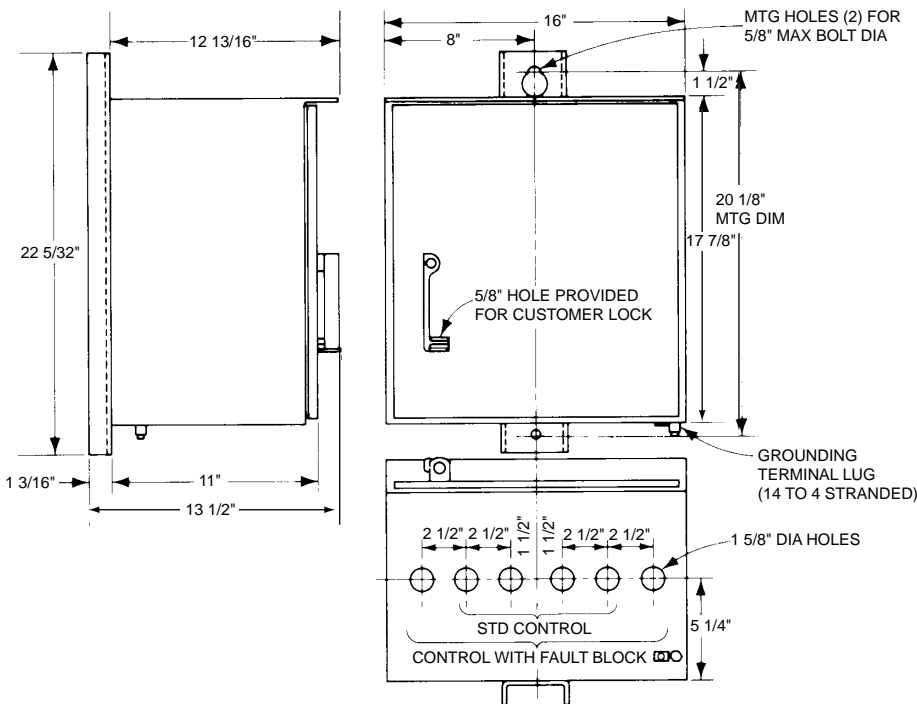
Figure 3. Outline and mounting dimensions.
