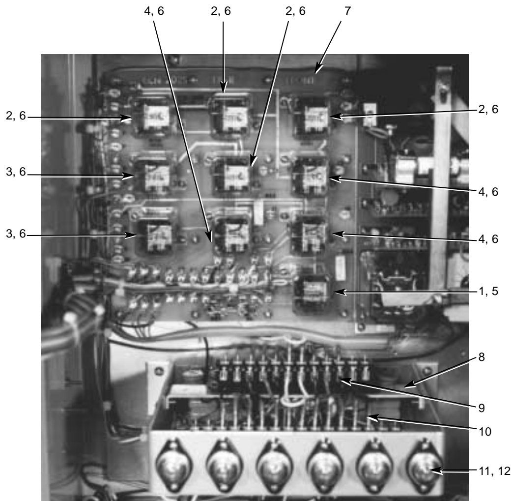
Figure 29. Back panel – replacement parts identification.
