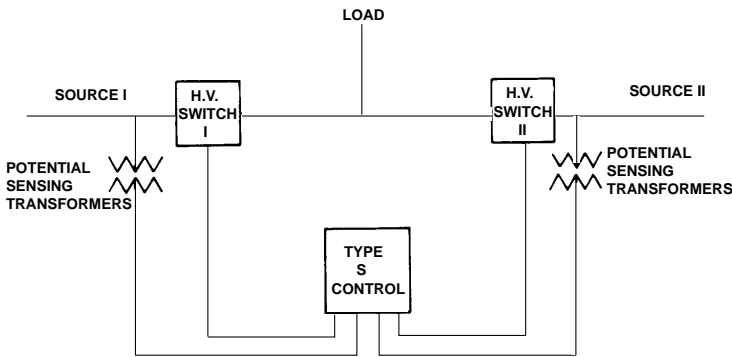
Figure 2. Typical Type S control load-transfer scheme.
