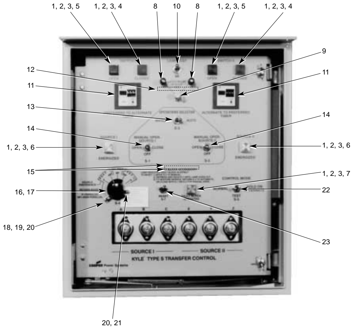
Figure 28. Front panel – replacement parts identification.
