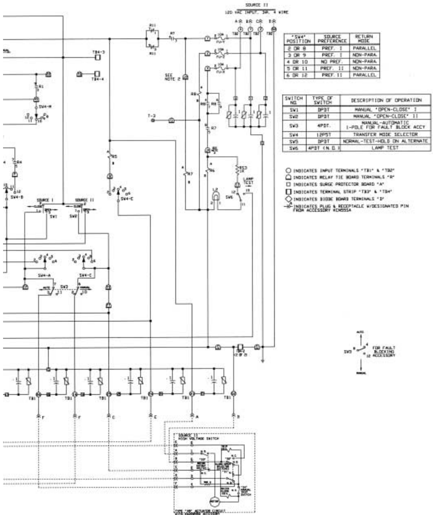
Figure 16b. Schematic diagram basic S control operating Types VR, VLR, VRV, TSC, or PST-9 switchgear (page 2 of 2).
