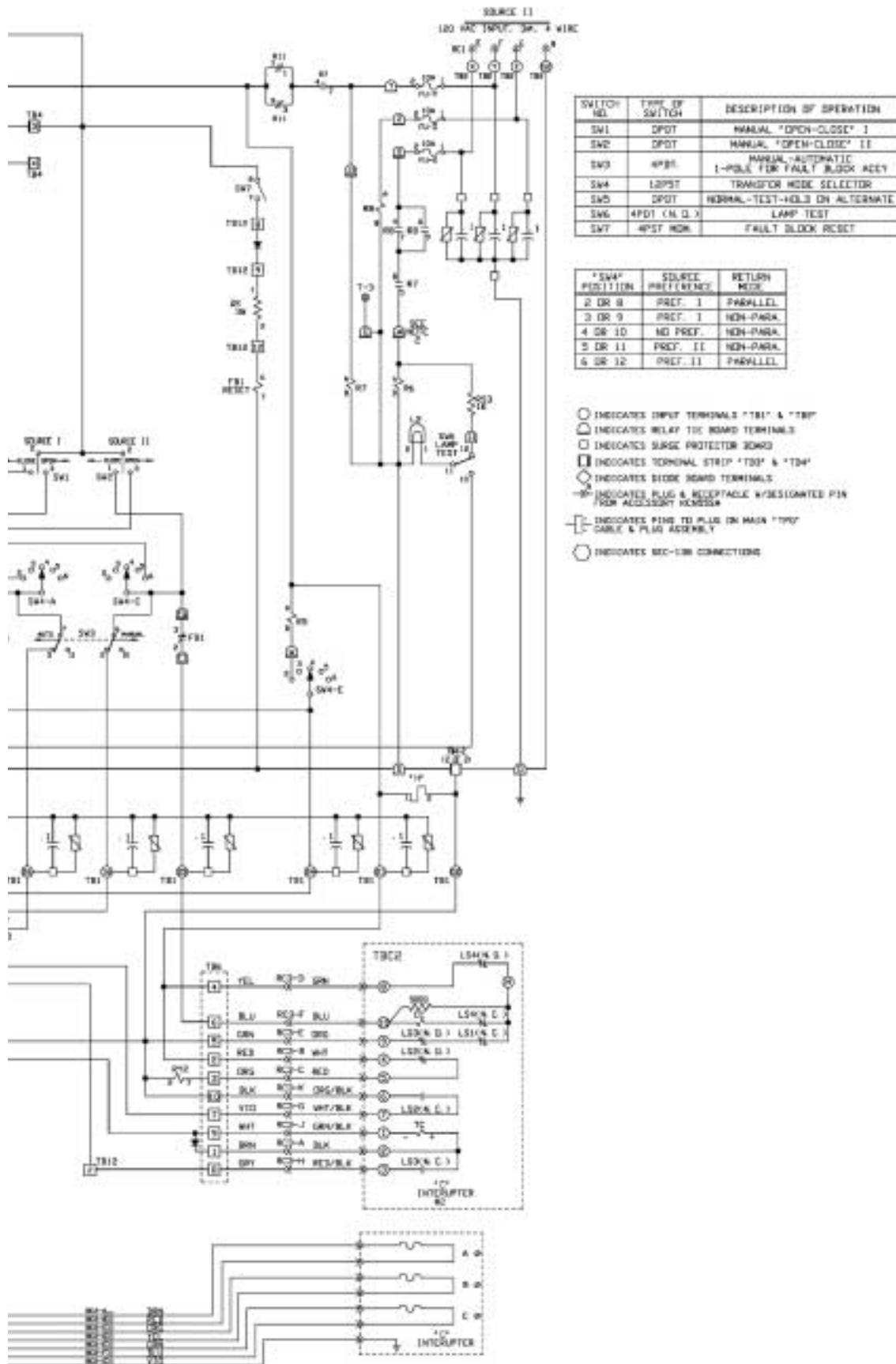
Figure 17a. Schematic diagram for Type S control operating Type PST-6 switchgear (page 2 of 2).
