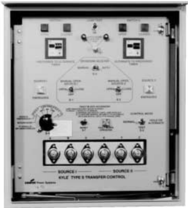
Figure 1. Kyle® Type S automatic load-transfer control.
