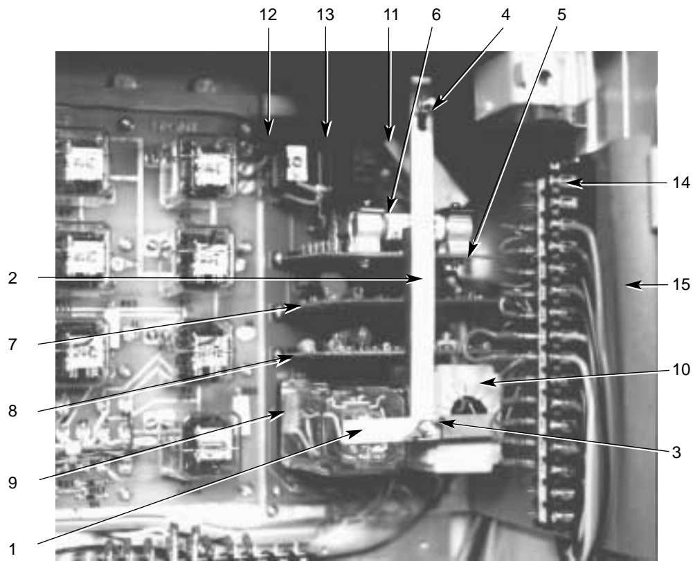
Figure 30. Fault block accessory – replacement parts identification.
