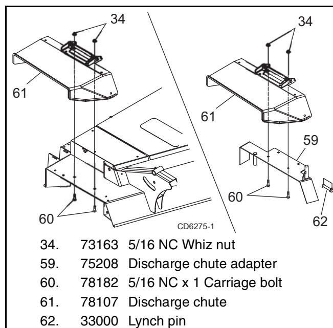
Figure 1. Discharge Removal
