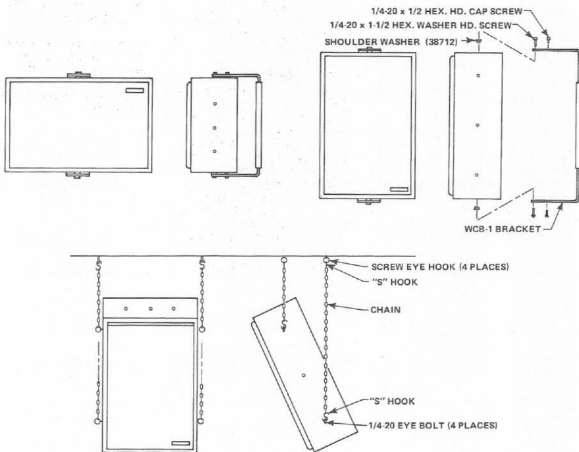
FIGURE 7 — System Mounting
