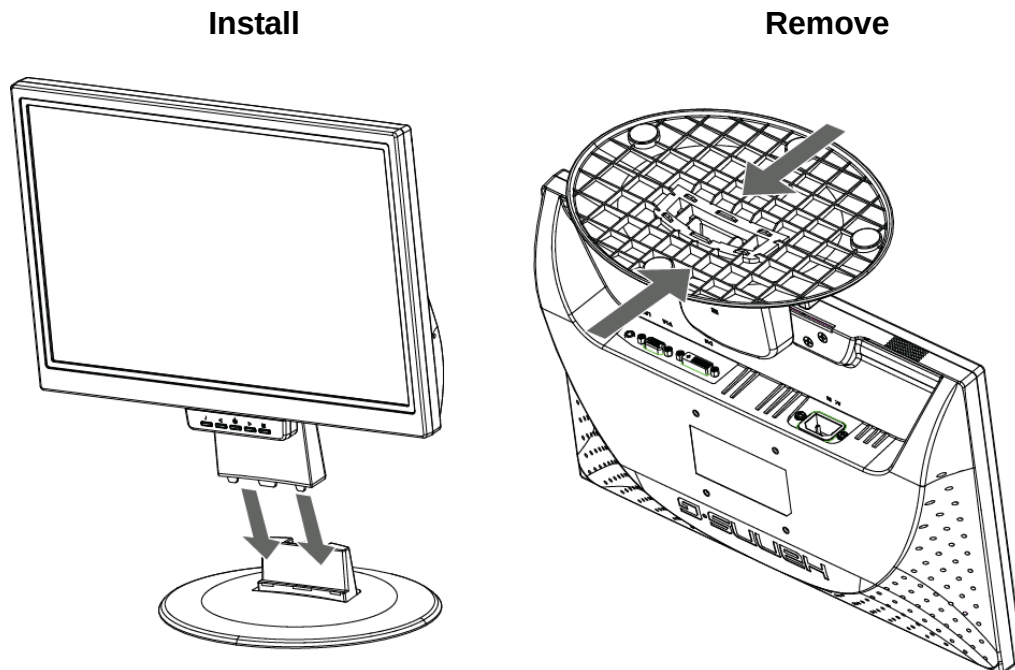
Figure.1. Installing and Removing the Base
