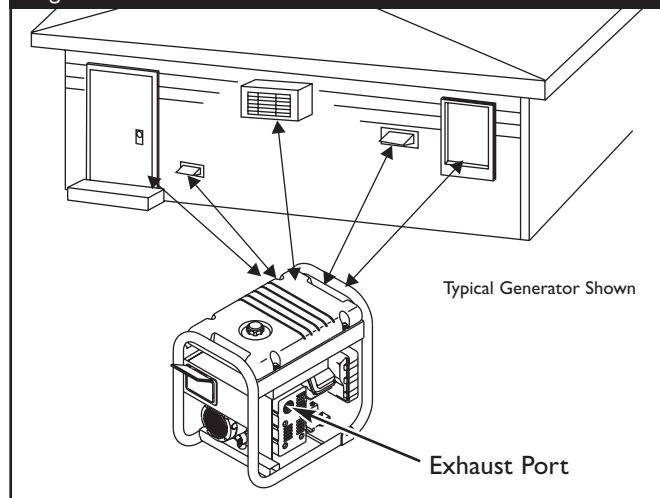
Figure 2 — Generator Clearance
