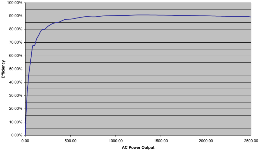
Figure A-1 Sun Tie XR efficiency curve
