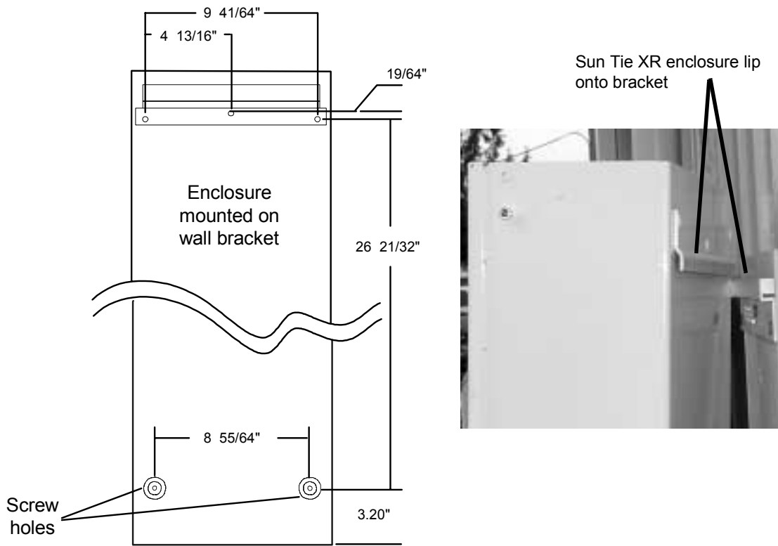
Figure 2-5 Enclosure mounting
