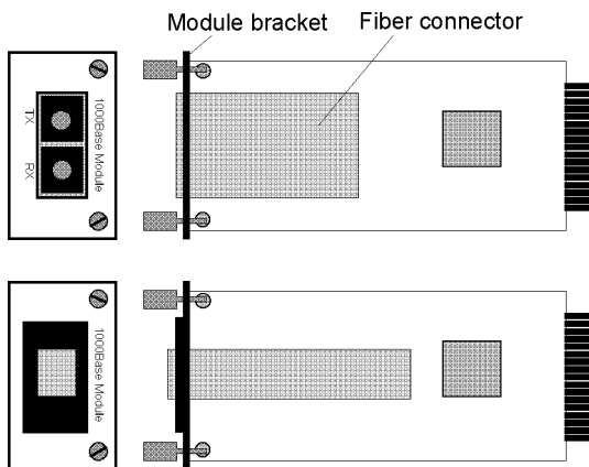
Gigabit Ethernet Modules (Top view)
