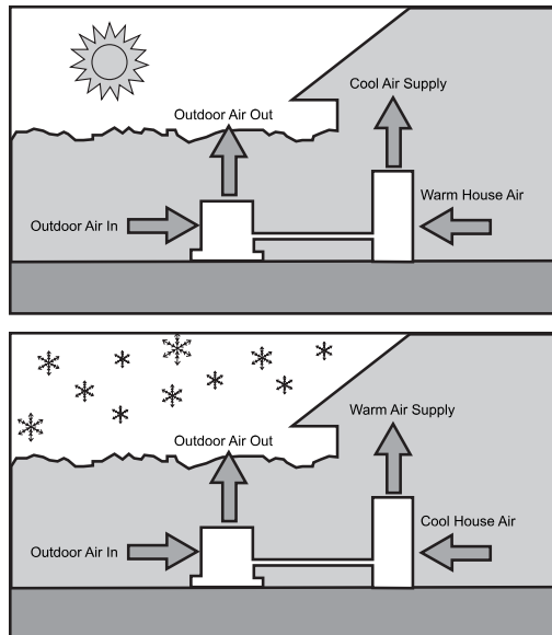
Fig.1 : Heat pump System
