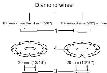
1. Lock nut 2. Abrasive cut-off wheel 3. Inner flange 4. Diamond wheel
