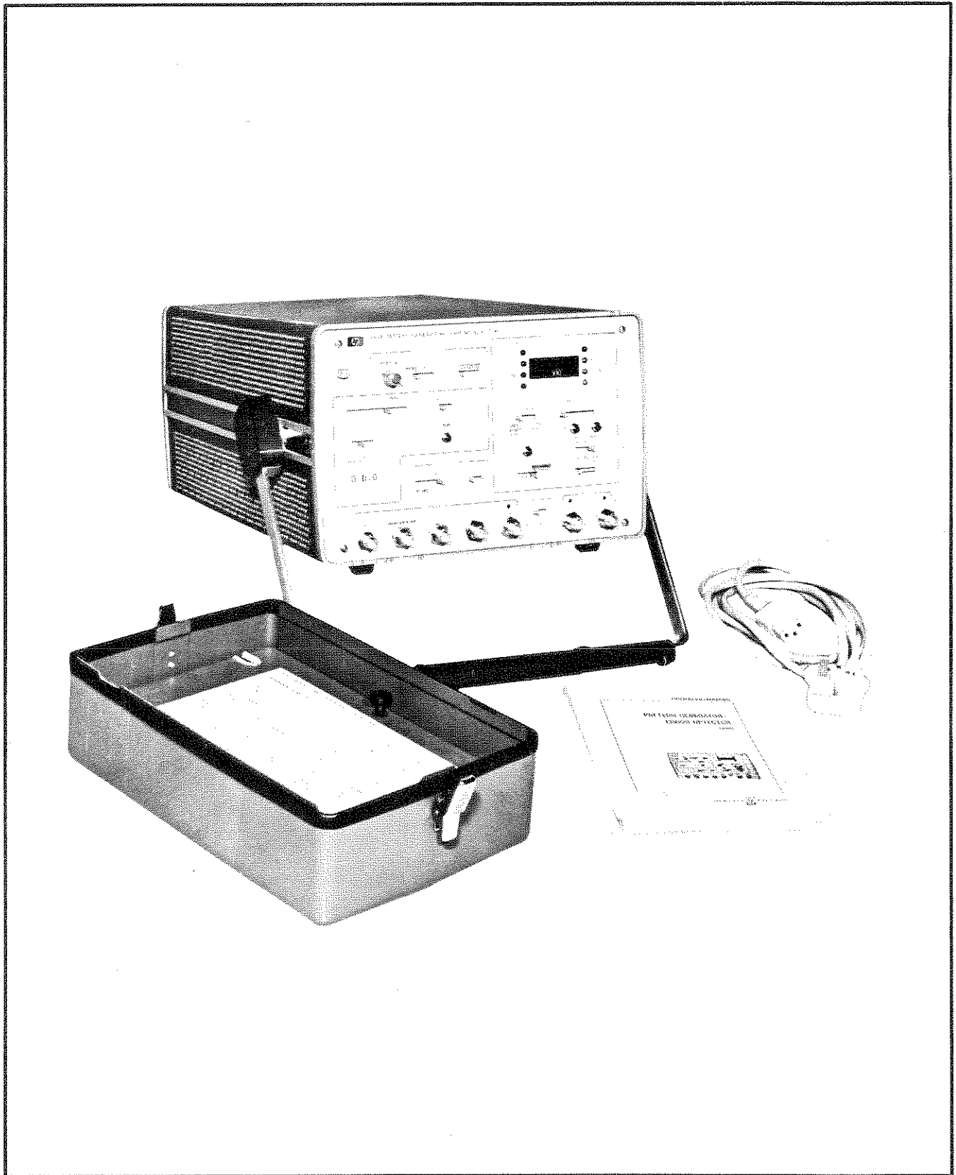
Figure 1-1 The 3780A Pattern Generator/Error Detector
