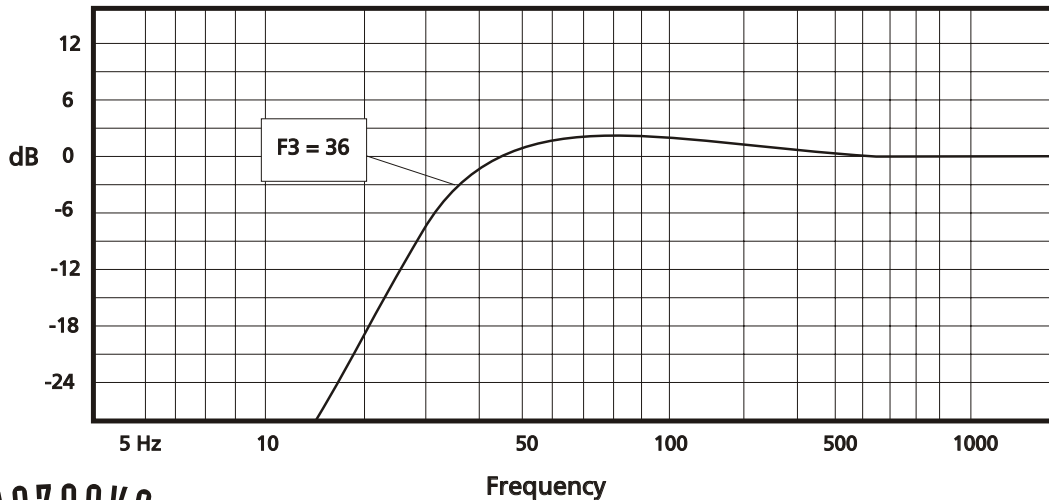
CSW1204 Amplitude Response (dB/Hz)
