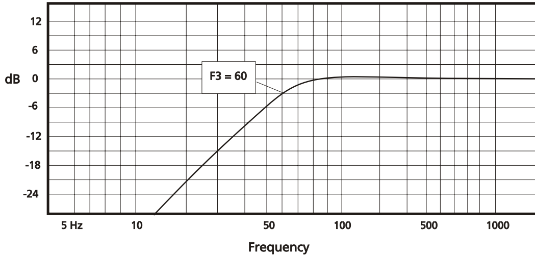
CSW1204 Amplitude Response (dB/Hz)
