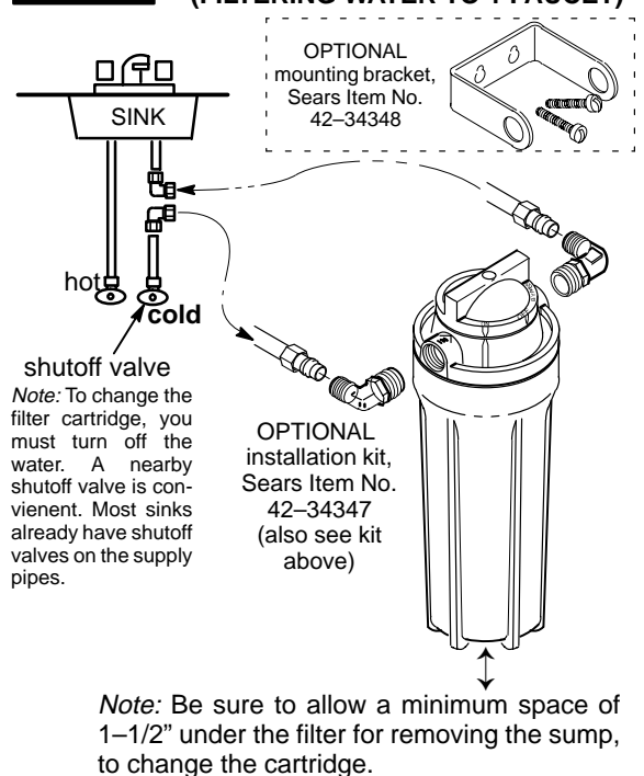
FIG. 4 UNDERSINK INSTALLATION (FILTERING WATER TO 1 FAUCET)
