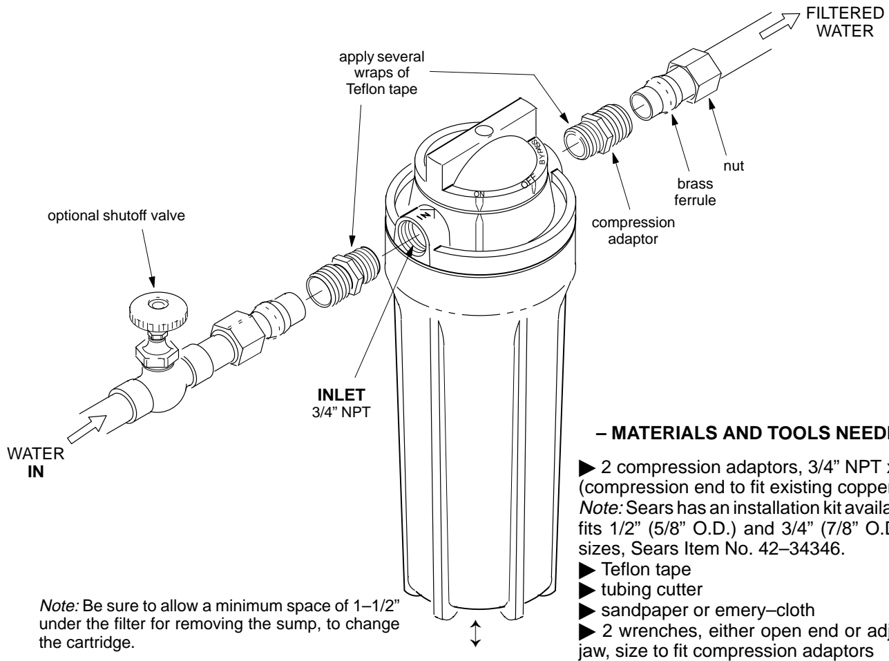
FIG. 1 INSTALLATION ON COPPER PLUMBING USING COMPRESSION FITTINGS
