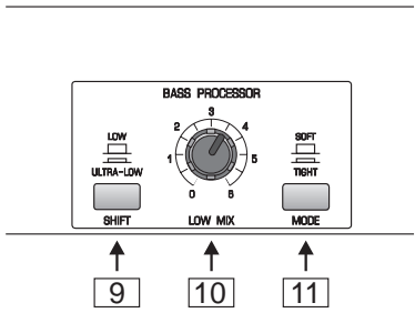
Fig. 4.3: Controls of the Bass Processor section
