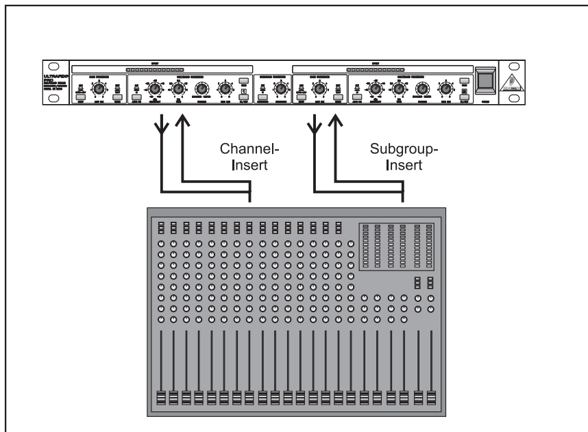
Fig. 6.1: Using the ULTRAFEX PRO as “in-line” processor
