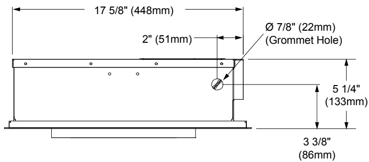
ELECTRICAL LOCATION SIDE VIEW
