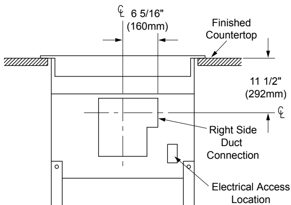
CABP3 DUCTED RIGHT (Inside Front Cabinet View)
