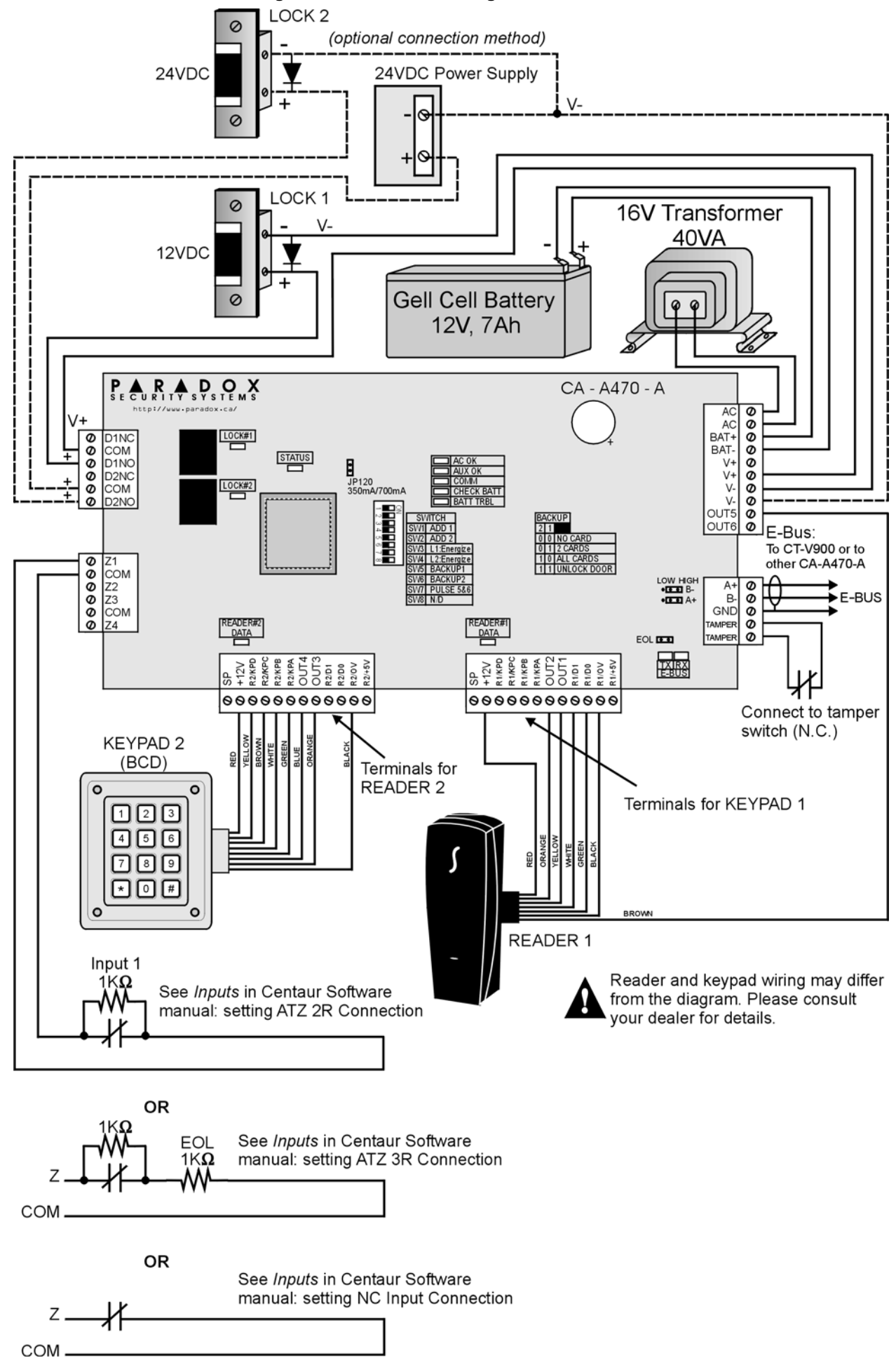
Figure 6: Connection drawing of the CA-A470-A
