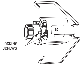
VARIFOCAL LENS
