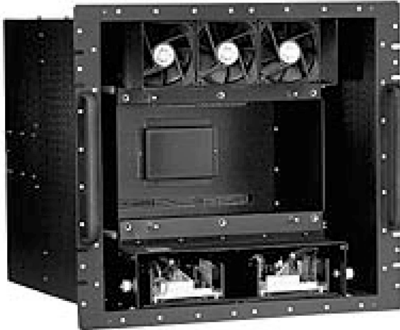
Basic Enclosure and Power Supply
