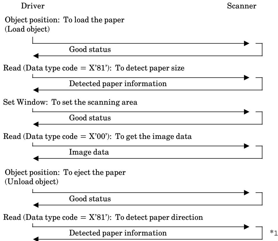
Figure D.1.1 Command sequence
