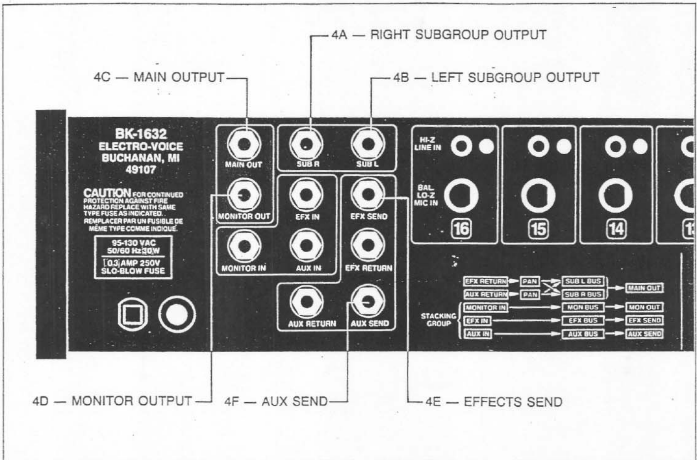
FIGURE 4 — Output Jacks
