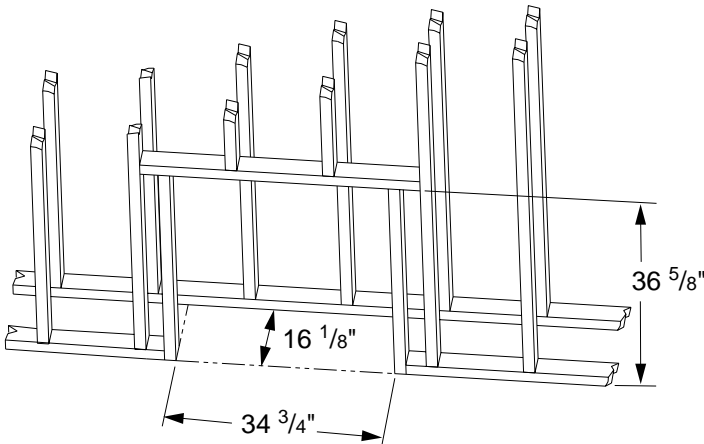
Figure 7 - Rough Opening for Installing in Wall
