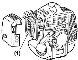
(1) Air filter
