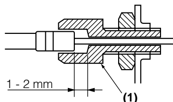
(1) Cable adjuster
