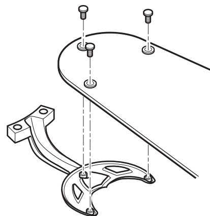
Figure 23 - Attaching the blade to the blade iron
