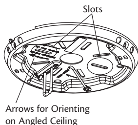
Figure 10 - Locating the slotted holes to use
