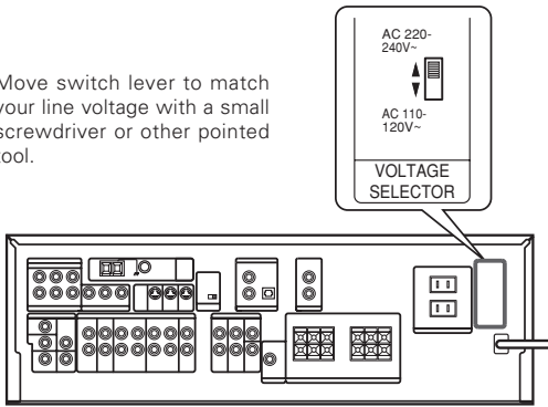
AC voltage selector switch
