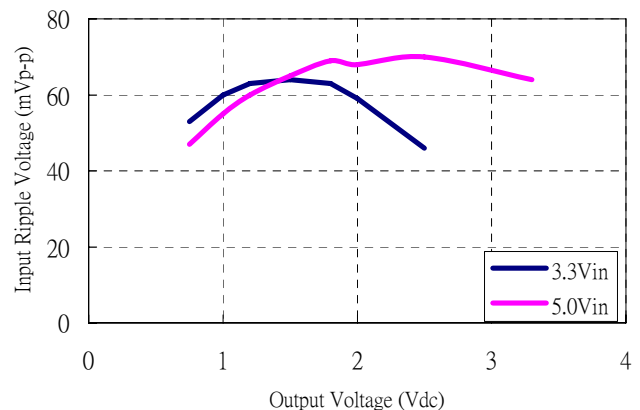
Figure 33: Input voltage ripple for various output models, I_o = 6A ( C_{IN} = 4 \times 100\mu F tantalum // 2x47µF ceramic)
