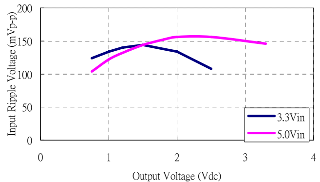
Figure 32: Input voltage ripple for various output models, I_o = 6A ( C_{IN} = 2 \times 100\mu F tantalum // 47µF ceramic)
