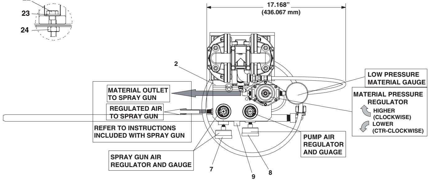
View B
