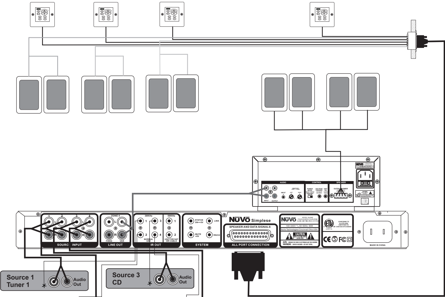
Simplese Wiring Diagram
