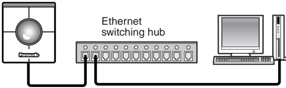
Ethernet cable (Category 5 straight cable)
