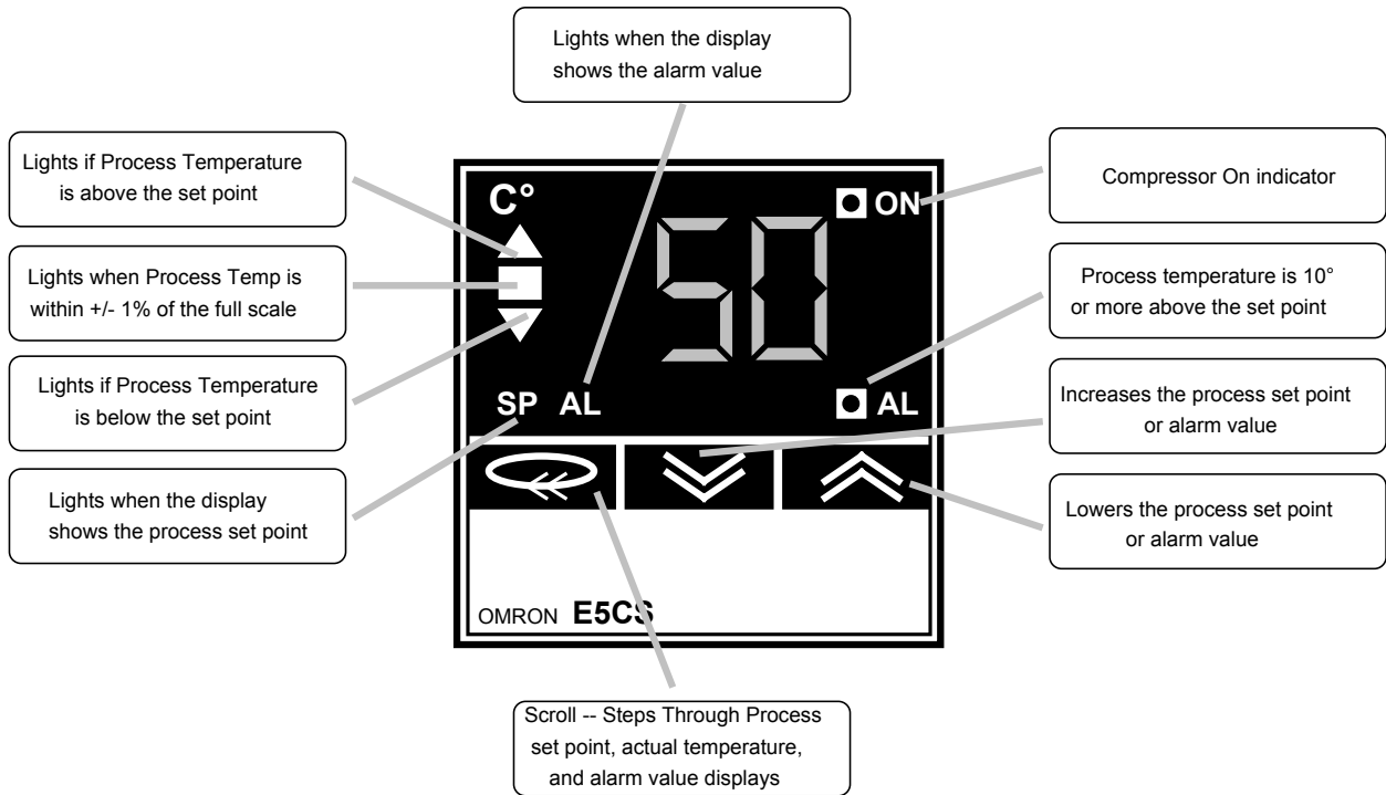
Figure 12 SMC Control
