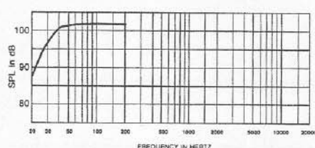
FIGURE 2E — EVX-180 and 184 Multiple-Driver Low-Frequency Performance: 4 Drivers in a 1132-L (40-ft³) Box or 2 566-L (20-ft³) Boxes in Close Proximity Tuned to 28 Hz
