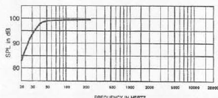
FIGURE 2D — EVX-180 and 184 Multiple-Driver Low-Frequency Performance: 2 Drivers in a 566-L (20-ft³) Box or 2 283-L (10-ft³) Boxes in Close Proximity Tuned to 30 Hz
