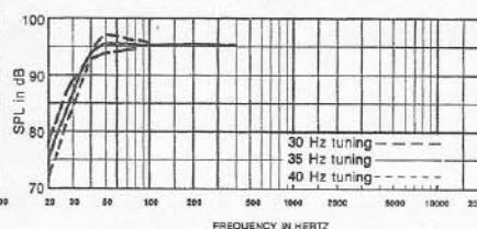
FIGURE 2B — EVX-180 and 184 Single-Driver Low-Frequency Performance: 283-L (10-ft³) Enclosure
