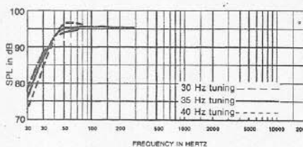
FIGURE 2A — EVX-180 and 184 Single-Driver Low-Frequency Performance: 223-L (8-ft³) Enclosure
