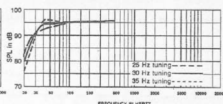
FIGURE 2C — EVX-180 and 184 Single-Driver Low-Frequency Performance: 336-L (12.5-ft³) Enclosure
