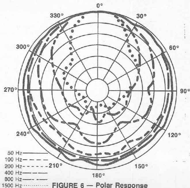
FIGURE 6 — Polar Response
