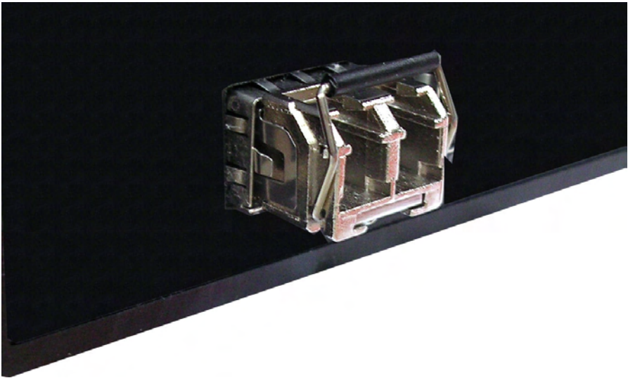
Figure 2.9: Transceiver Inserted
