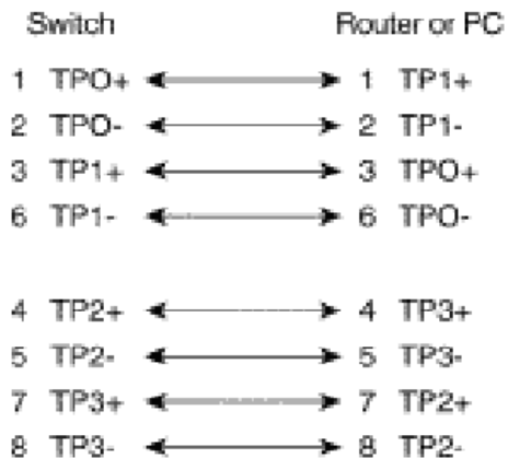
Straight through cables schematic
