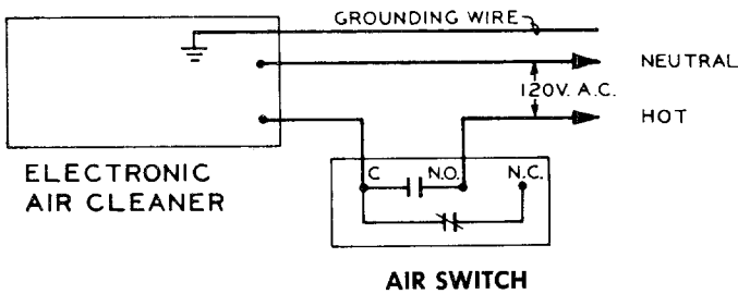
Fig. 2 - Typical Air Cleaner Installation.
