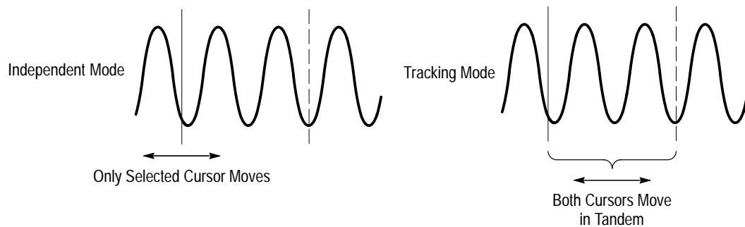
Figure 3-62: Cursor Modes
