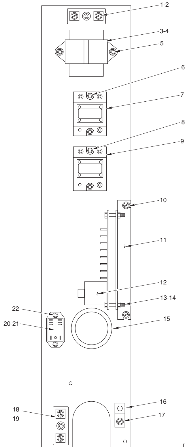
ELECTRICAL COMPONENT PANEL (PROGRAMMABLE)
