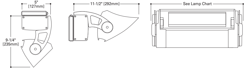
LAMP CHART - Remote
