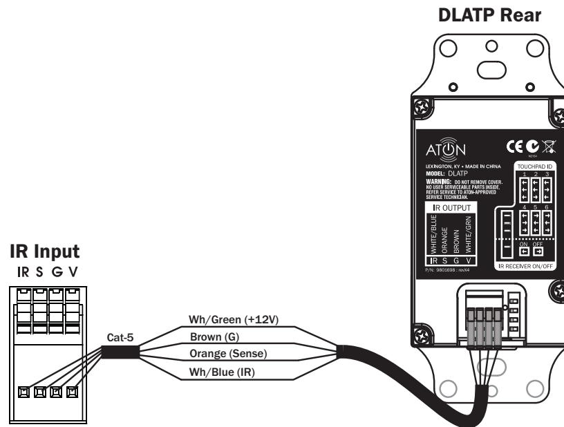
Figure 3-5: DLATP Connections
