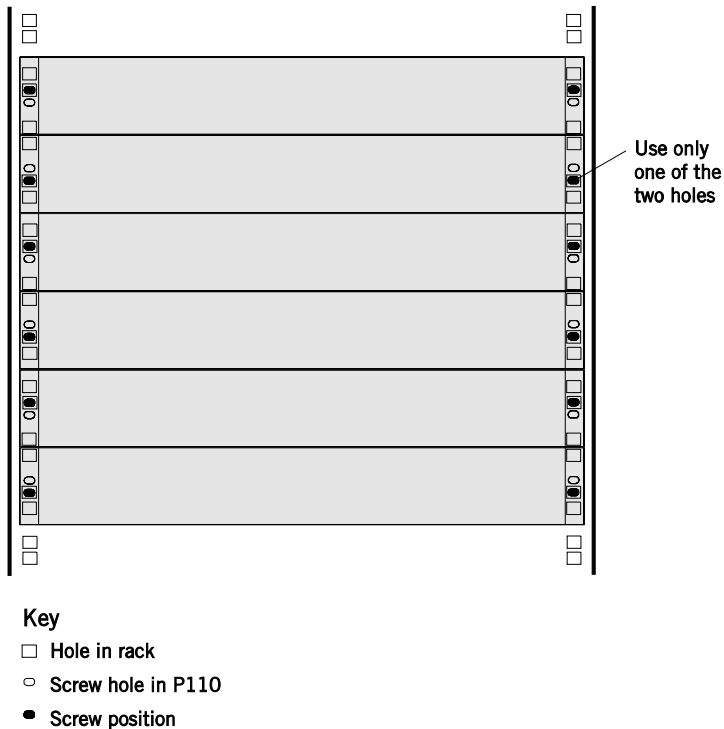
Figure 3 P110 rack mounting arrangement
