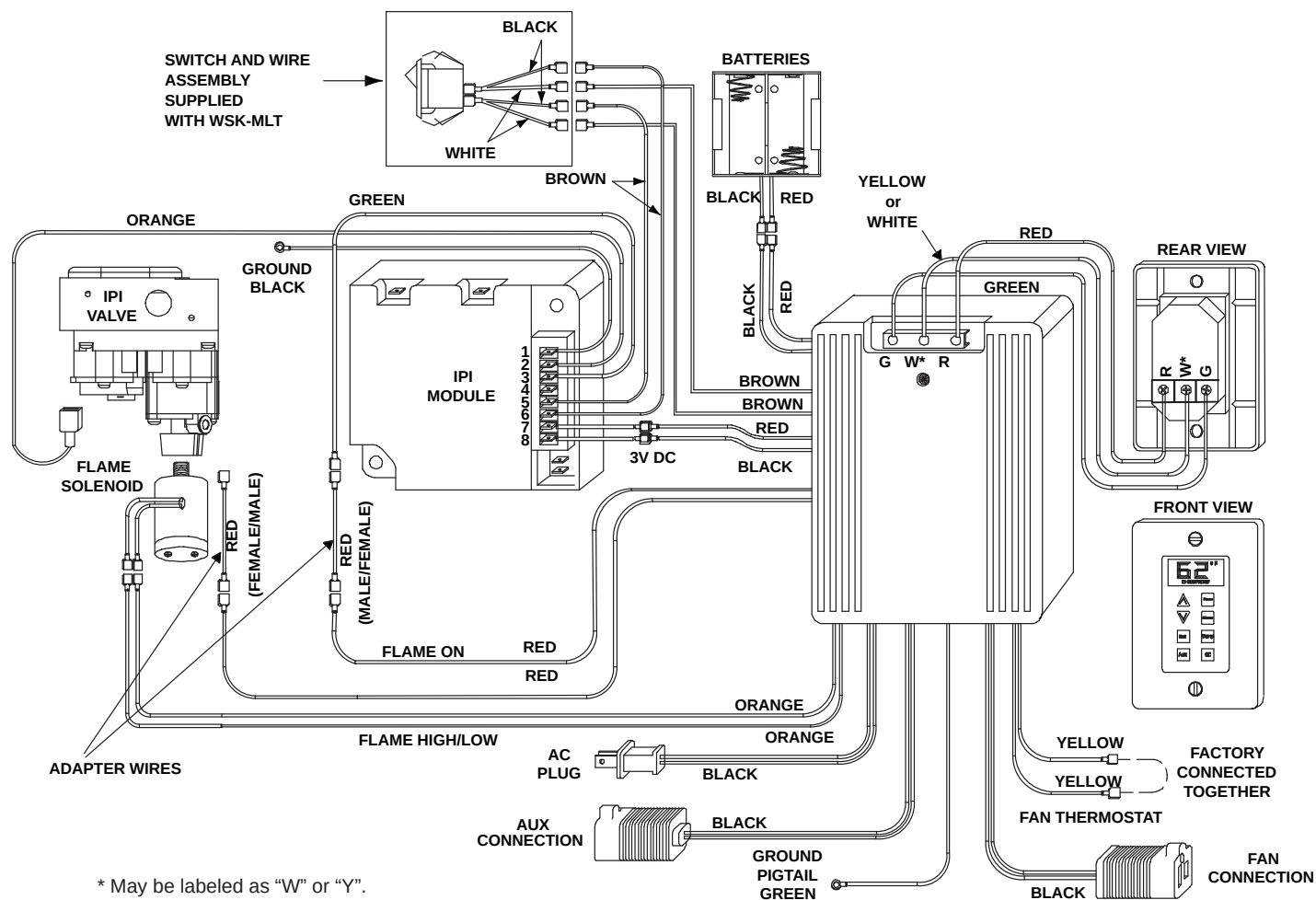
Figure 5. Intellifire (IPI) Wiring Diagram
