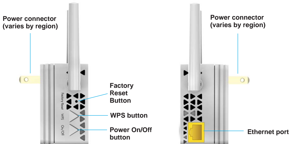
Figure 2. Side panel buttons and port
