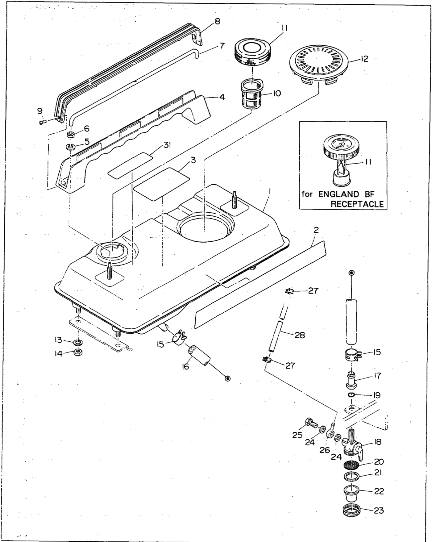
FIG. 1 FUEL TANK
