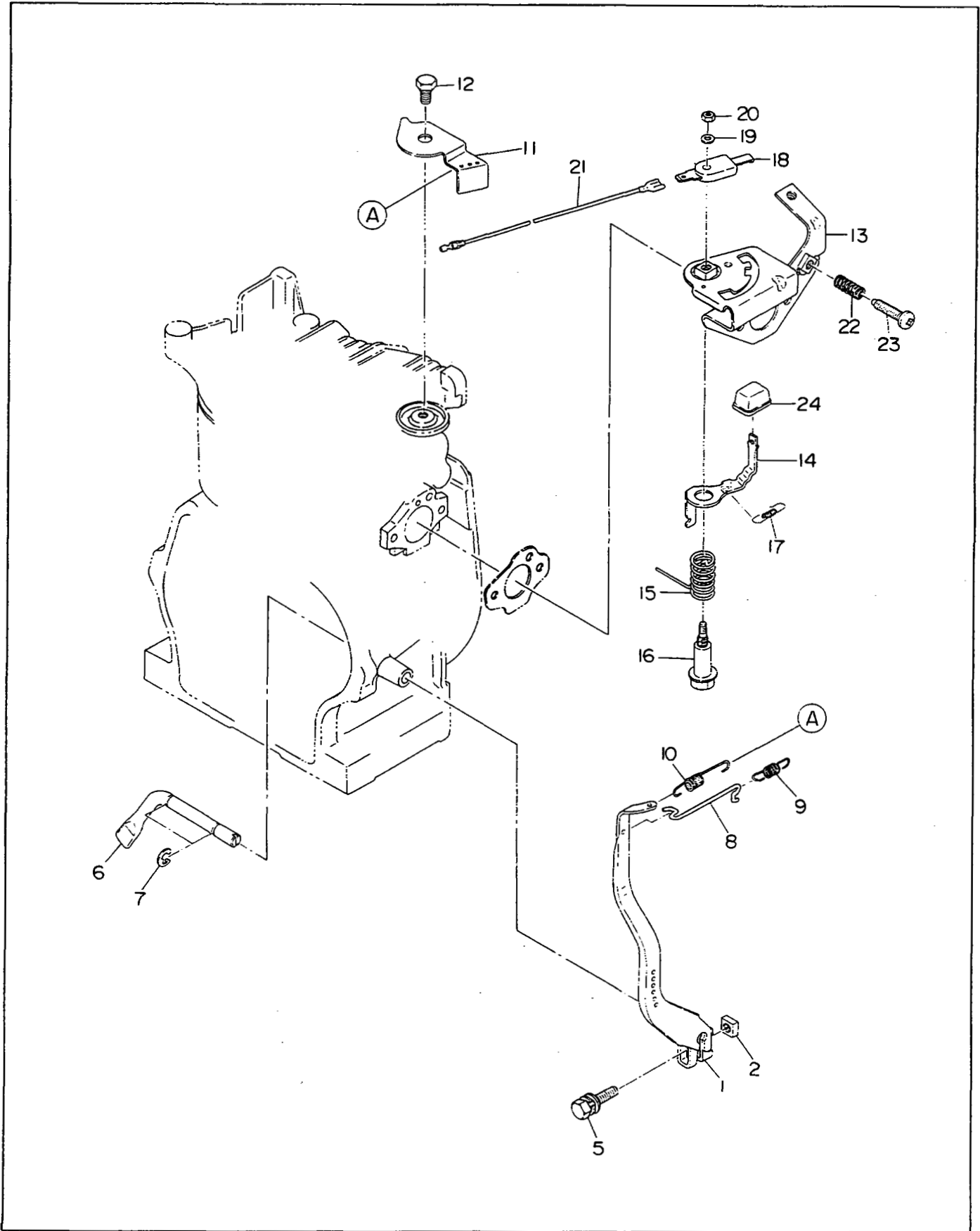
FIG. 7 GOVERNOR
