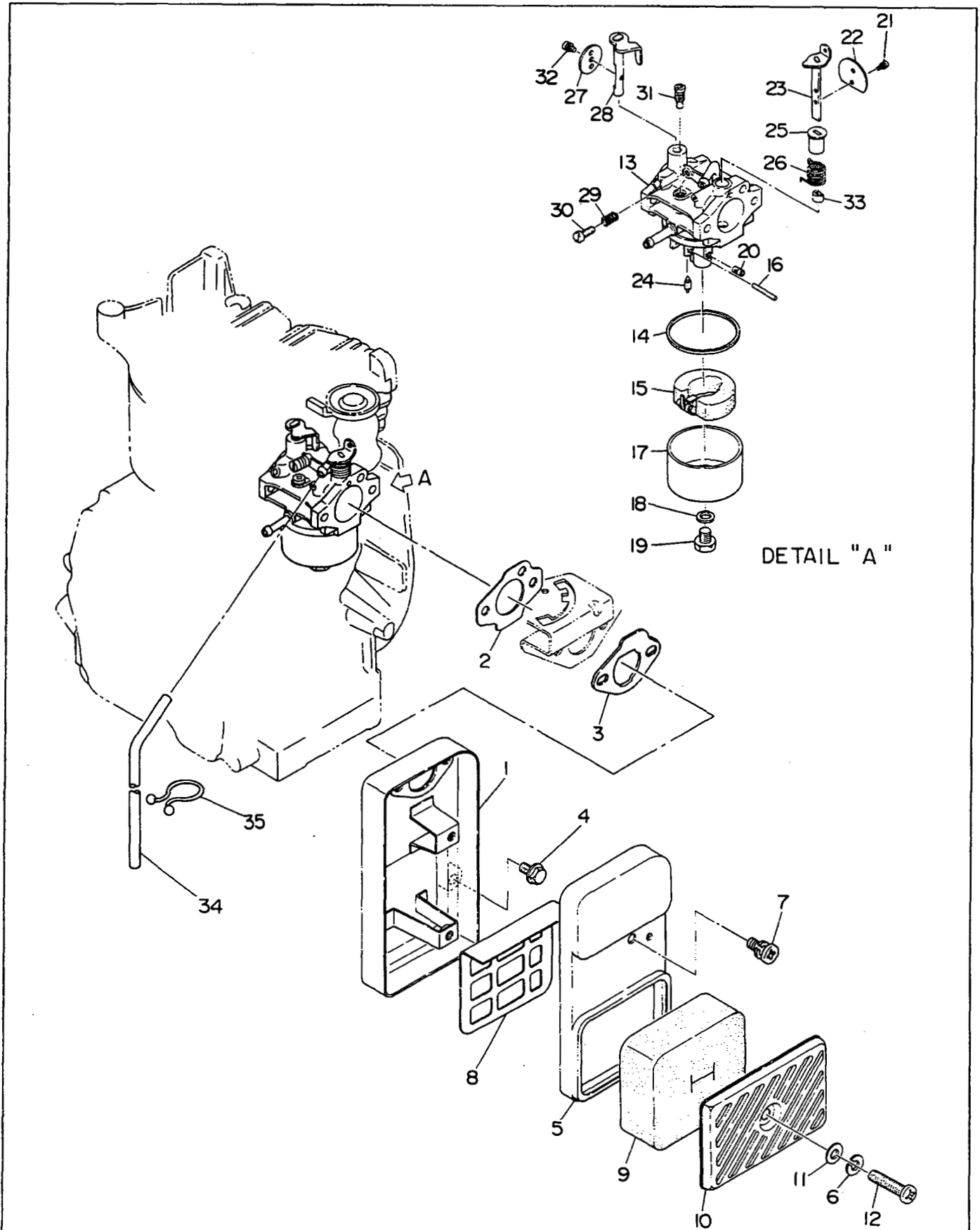
FIG. 9 CARBURETOR and AIR CLEANER
