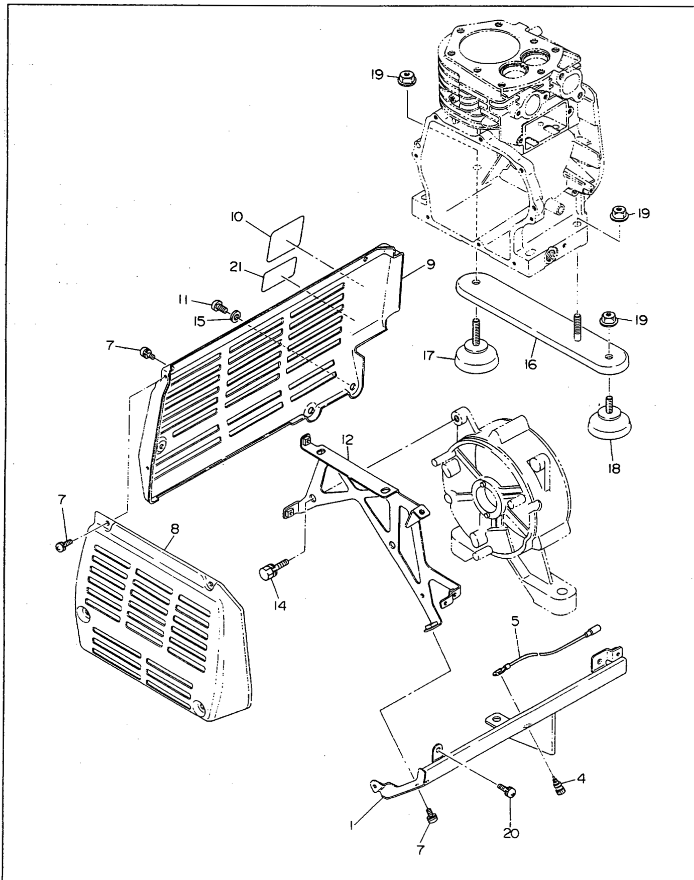
FIG. 4 COVER
