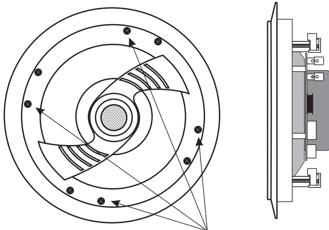
Mounting screws (4)
