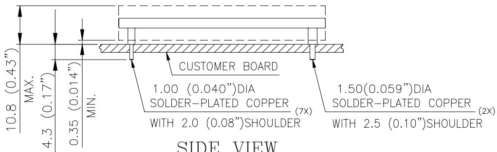
SIDE VIEW
