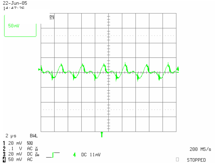
Figure 12: Output voltage ripple at 36V input voltage and rated load current (50 mV/div). Load capacitance: 1 \mu F ceramic capacitor and 10 \mu F tantalum capacitor. Bandwidth: 25 MHz. Scope measurements should be made using a BNC cable (length shorter than 20 inches). Position the load between 51 mm to 76 mm (2 inches to 3 inches) from the module.
