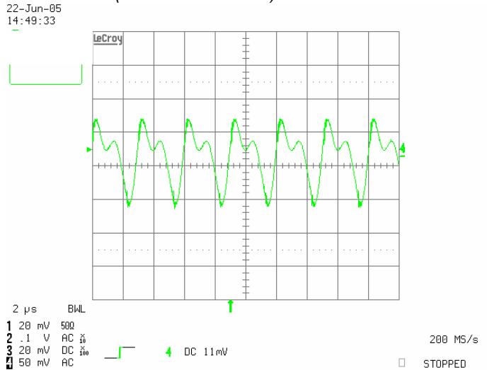
Figure 12: Output voltage ripple at 36V input voltage and rated load current (50 mV/div). Load capacitance: 1 \mu F ceramic capacitor and 10 \mu F tantalum capacitor. Bandwidth: 25 MHz. Scope measurements should be made using a BNC cable (length shorter than 20 inches). Position the load between 51 mm to 76 mm (2 inches to 3 inches) from the module.
