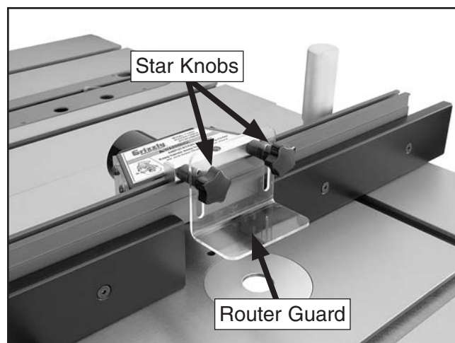
Figure 18. Router guard installed.
