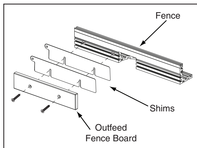
Figure 15. Shim installation for full edge routing.
