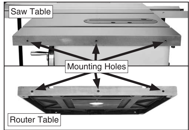
Figure 6. Required mounting holes in the router and saw tables.
