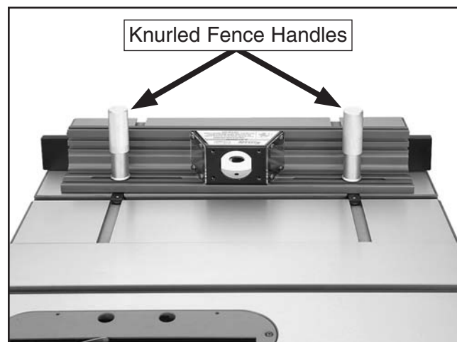
Figure 14. Knurled fence handles installed.
