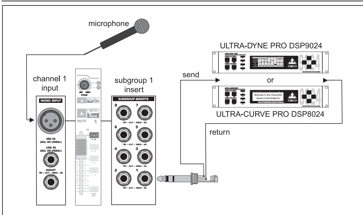
Fig. 5.2: Inserting an external EQ/dynamics processor post channel EQ
