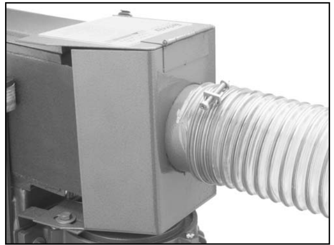
Figure 20. Dust port connected to dust collection system.
