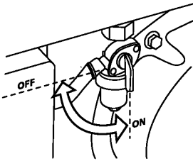
FIGURE 13: Fuel Valve Lever — ON/OFF position
