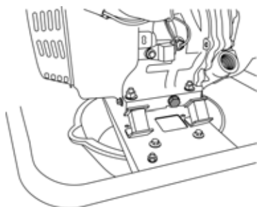
FIGURE 21: Oil Drain Bolt
