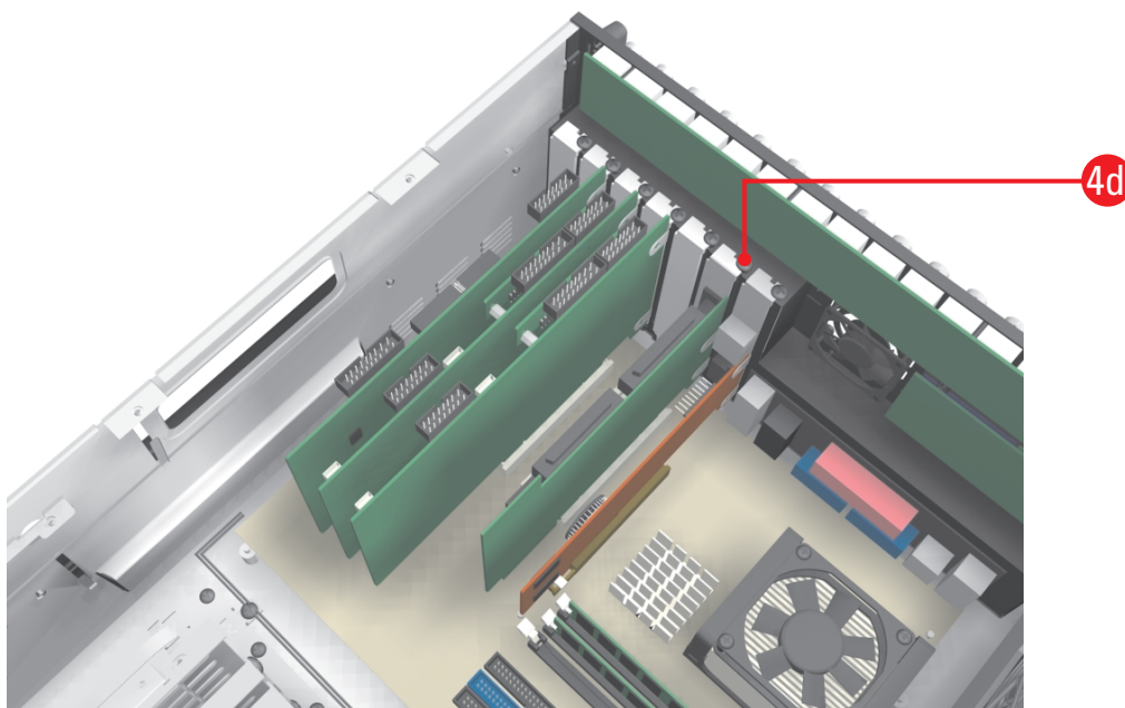
Figure 12. Securing the DX8000-ISCI SCSI Card
