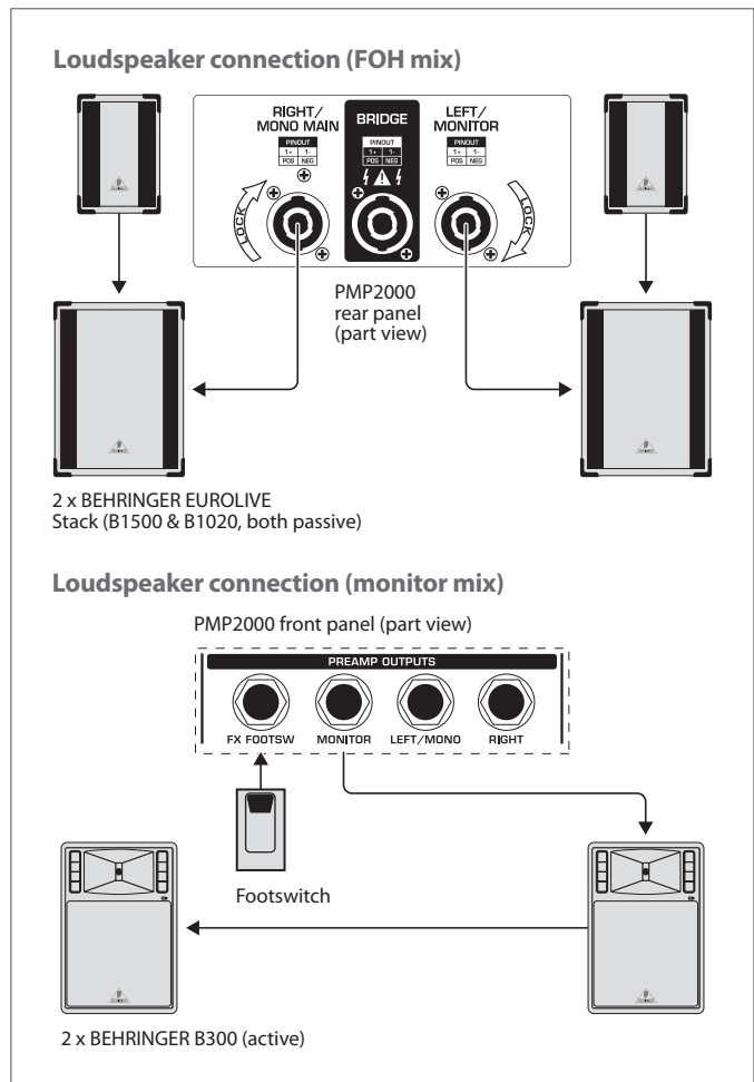
Fig. 5.1: PMP2000 as stereo amplifier (example)
