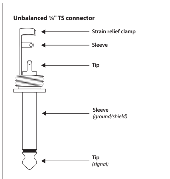
Fig. 4.1: 1/4" mono plug
