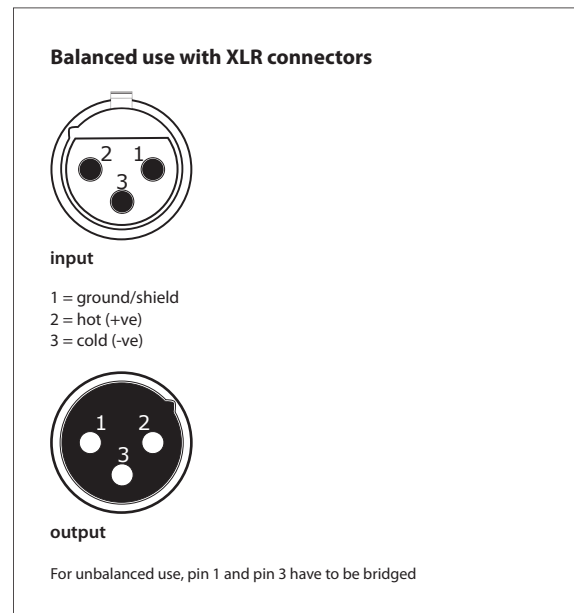
Fig. 4.3: XLR connectors
