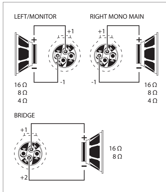
Fig. 4.6: PMP2000 loudspeaker connector assignment
