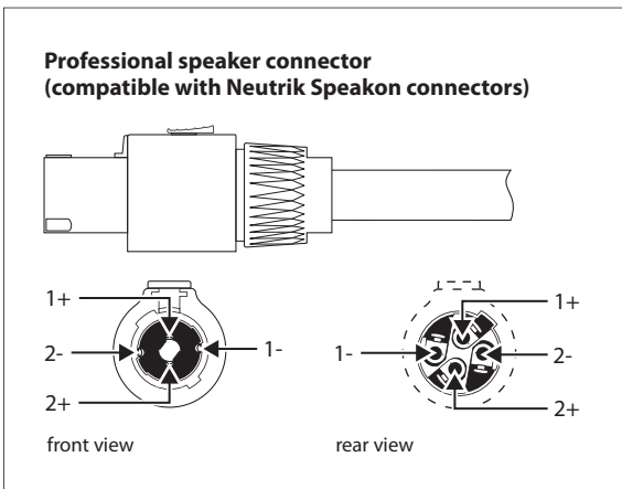
Fig. 4.5: Loudspeaker connector
