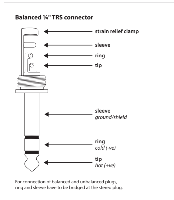
Fig. 4.2: 1/4" stereo plug
